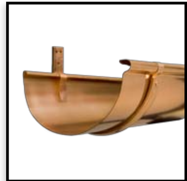
Classic Bar Bracket & Scroll Bar Bracket 5", 6" & 8", Copper & Aluminum, 1" wide x 3/16" thick
